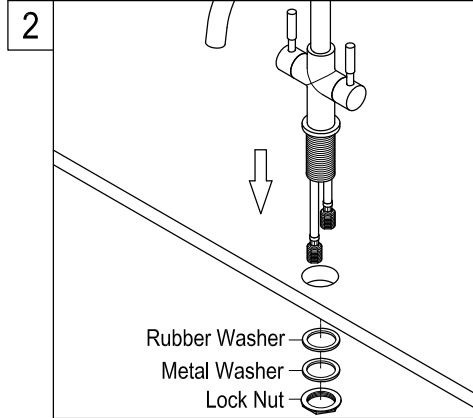
2. Insert the inlet shanks through the sink holes, and press down. Assemble the washers and lock nuts on the inlet shanks, and then tighten the nuts by wrench.
